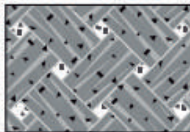
Loose graphite in standard PTFE braiding
